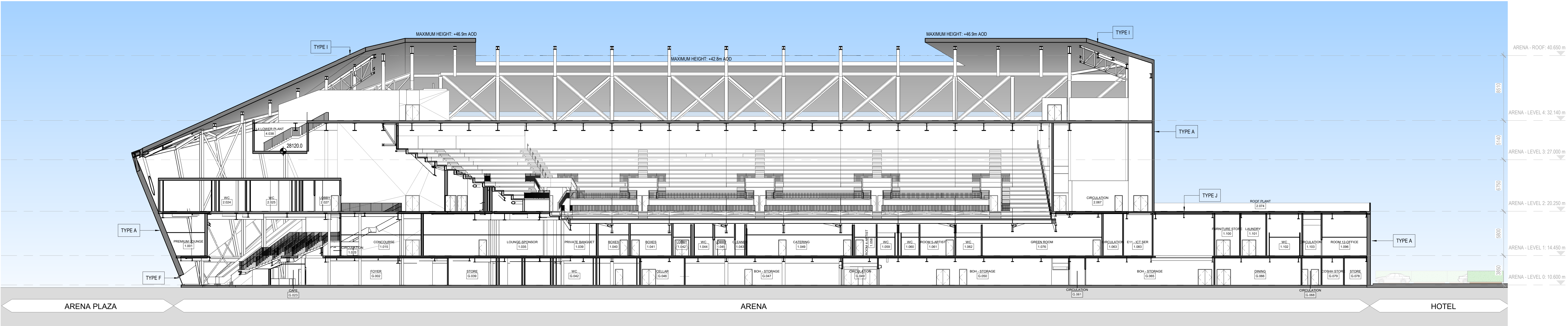
ARENA NORTH SOUTH LONGITUDINAL SECTION - WEST 1: 200
