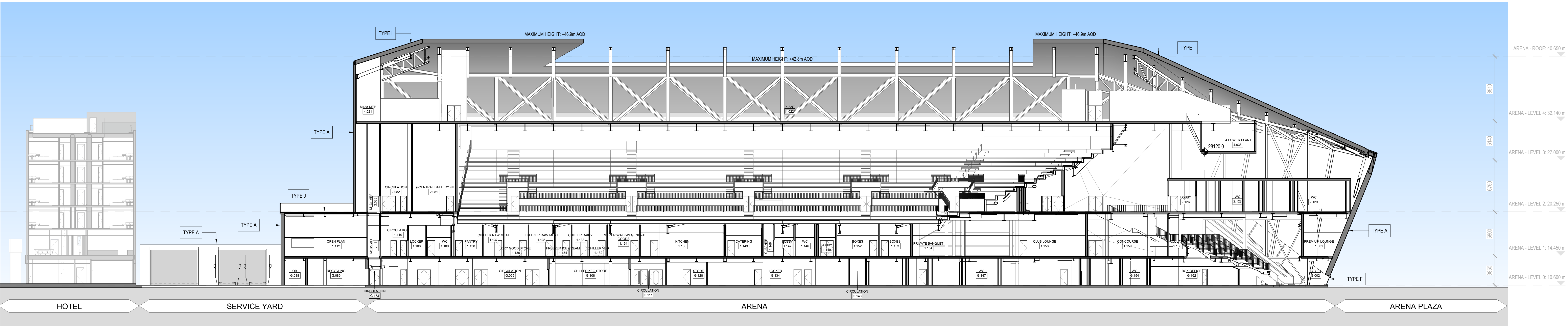
ARENA NORTH SOUTH LONGITUDINAL SECTION - EAST 1: 200
