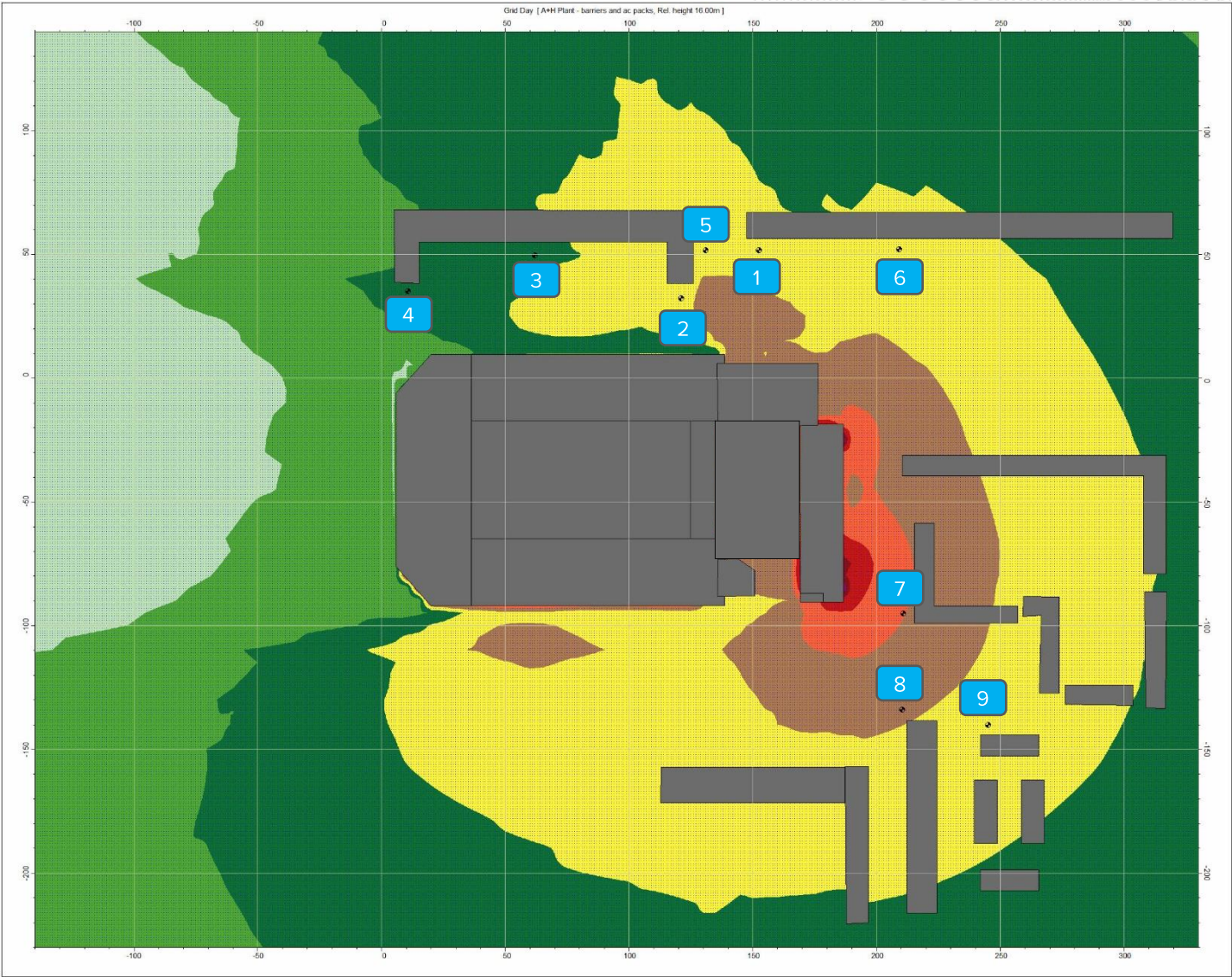
CARDIFF ARENA – STAGE 3 – NOISE BREAK-OUT PREDICTIONS AT 16m
