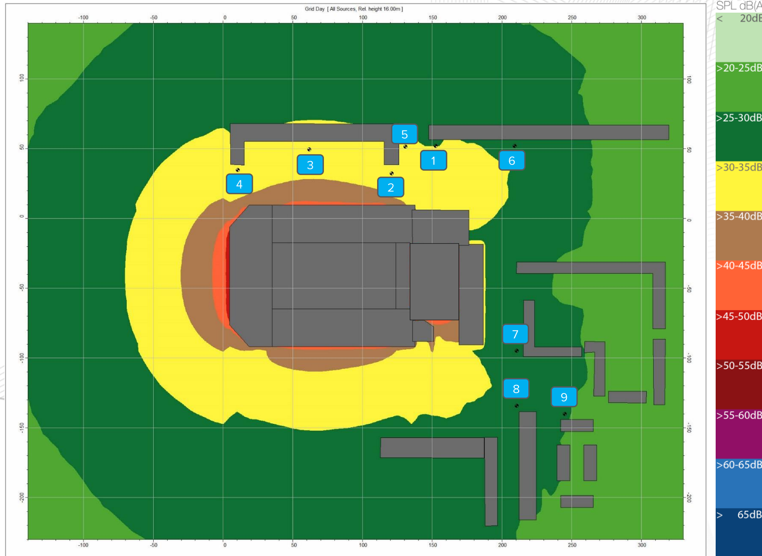
CARDIFF ARENA – STAGE 3 – NOISE BREAK-OUT PREDICTIONS AT 16m
